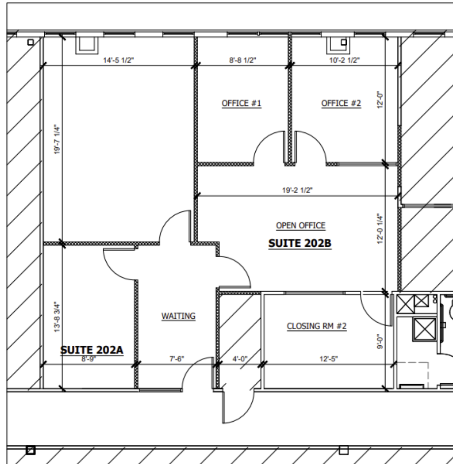
EXHIBIT A - SUITE 202B 3/16" = 1'-0"
